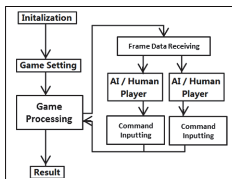
Fig. 1. Game engine's architecture and the processing flow.
