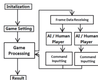
Fig. 1. Game engine's architecture and the processing flow.
